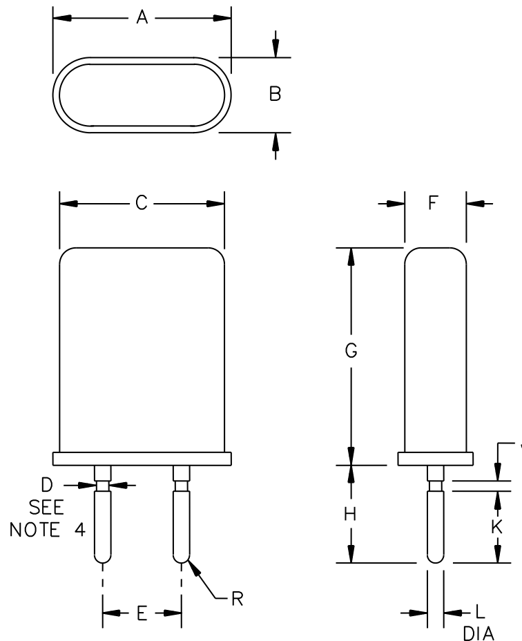
FIGURE 1. Crystal unit - CR82/U.
