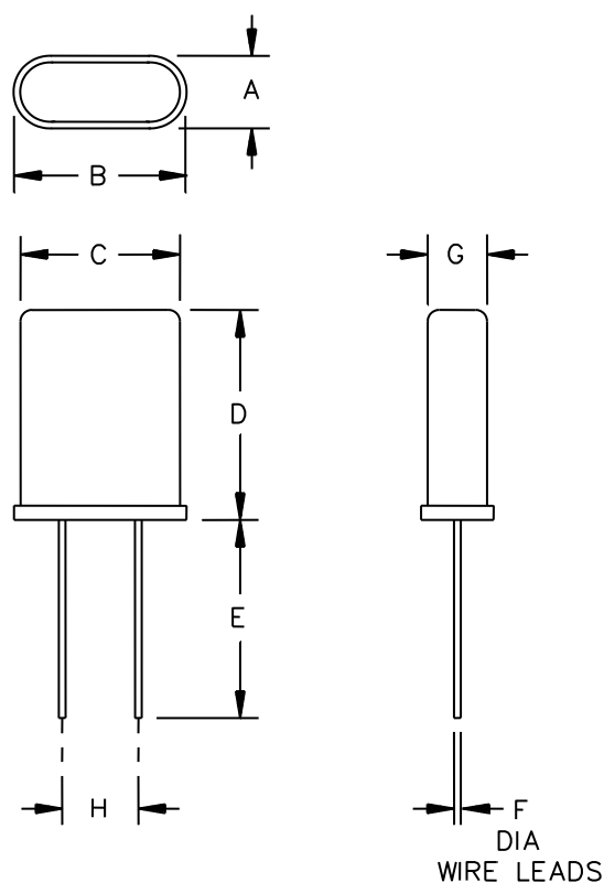
FIGURE 1. Crystal unit - CR56/U.
